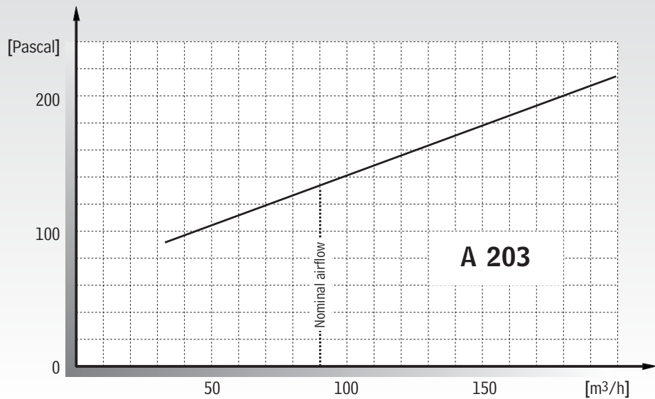
Pressure Drop on Airflow A 203:
